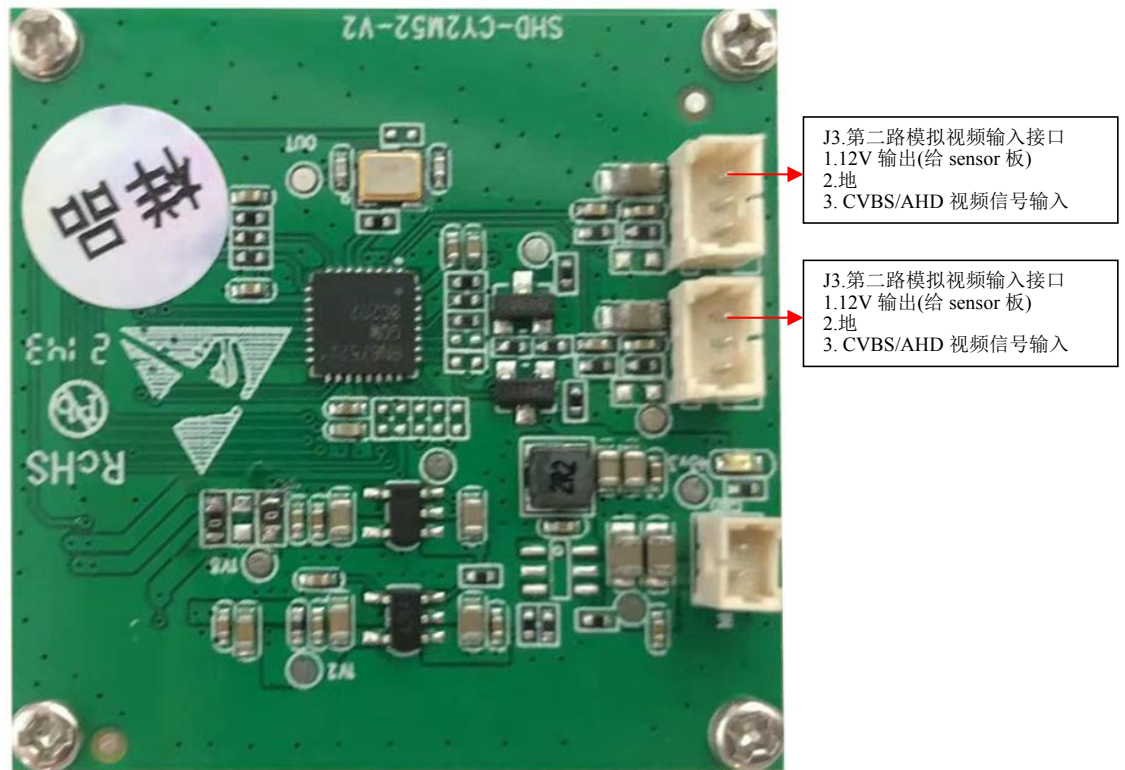
4. AHD+CVBS 接口板背面定义:
